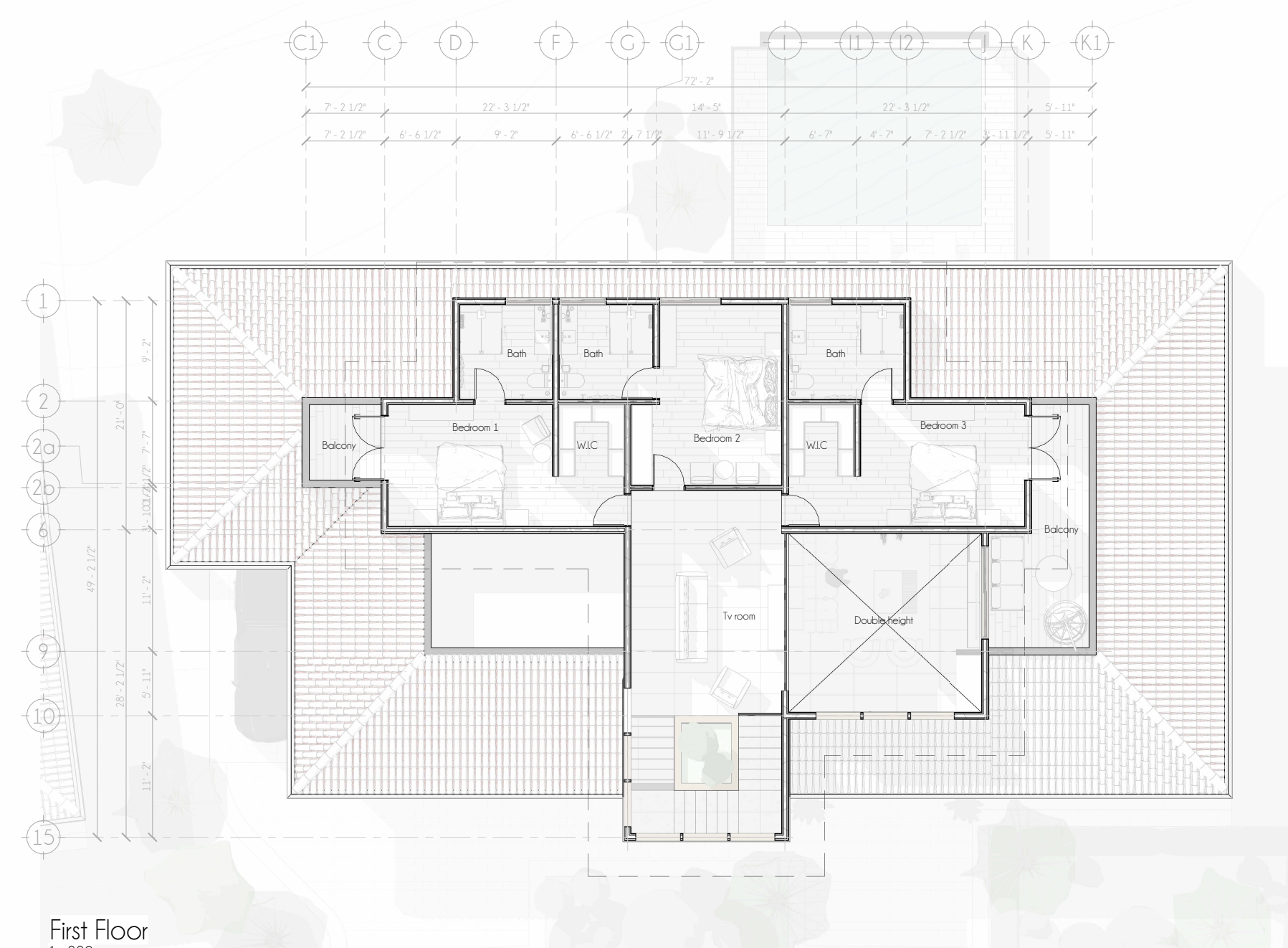
First Floor 1:220
